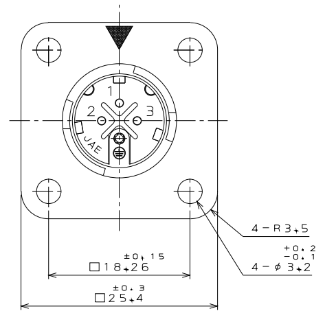
Mating Side
