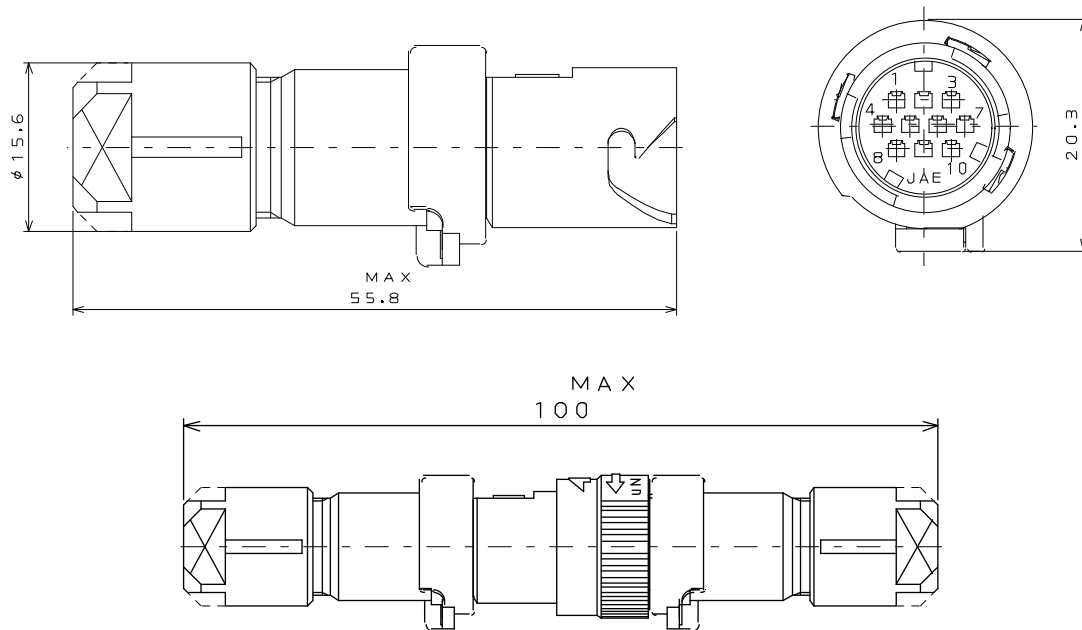
Drawing (when mated)
