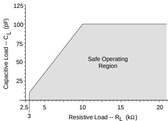
Figure 2. Maximum Loading
