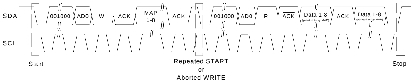
Figure 23. I²C Read
