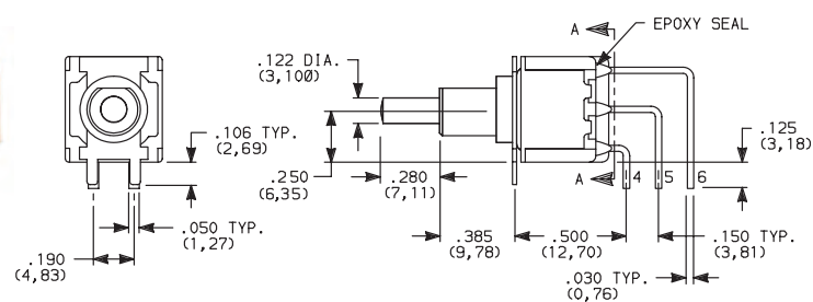
8261SH9AV2BE2 DPDT
