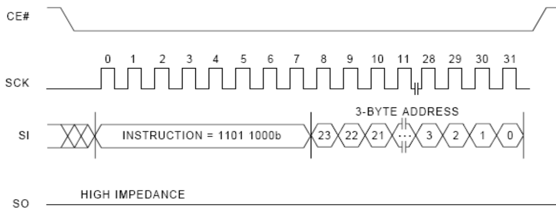
Figure 24. Block Erase Sequence
