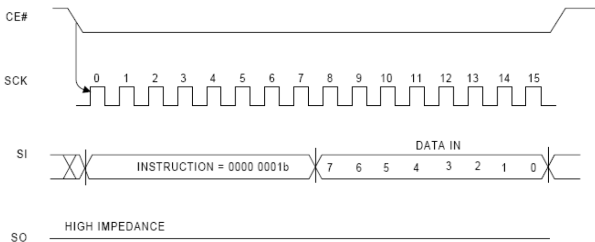
Figure 11. Write Status Register Sequence
