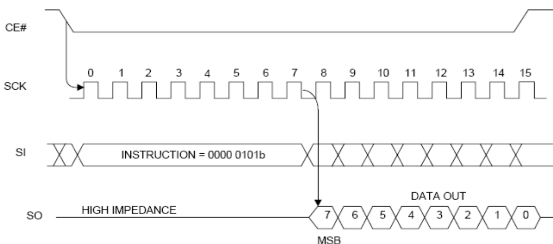
Figure 10. Read Status Register Sequence
