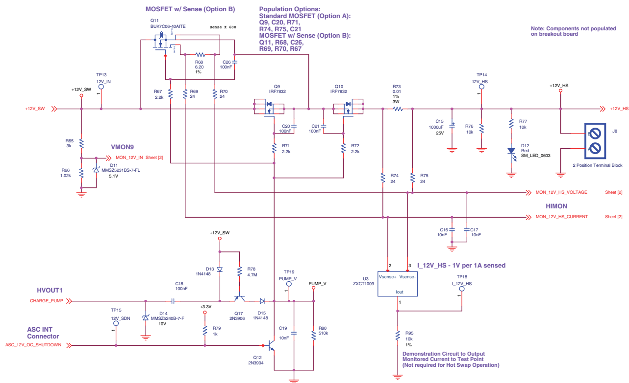
Figure 19. 12 V HS Circuit
