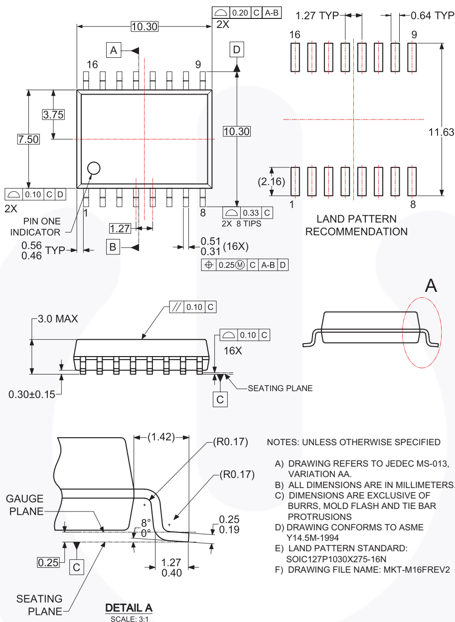
Figure 60. 16L SOIC Wide Body
