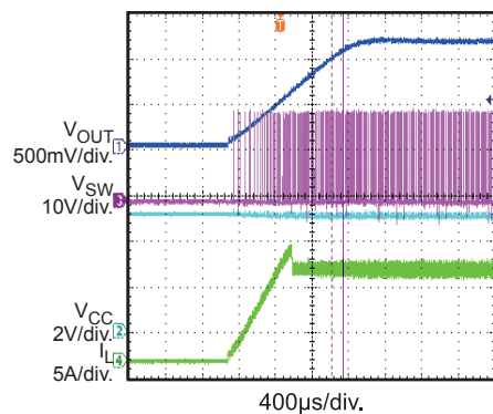
Thermal Recovery
