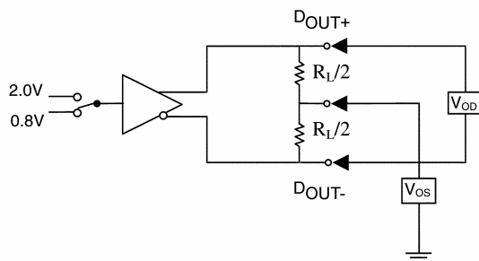
Figure 4. Differential Driver DC Test Circuit
