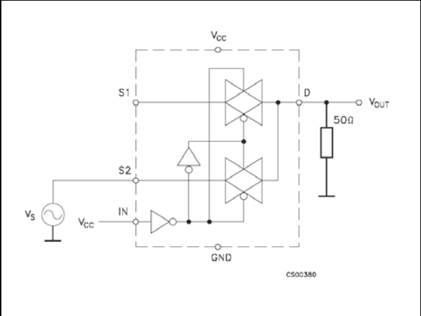
Figure 6. Channel-to-channel crosstalk
