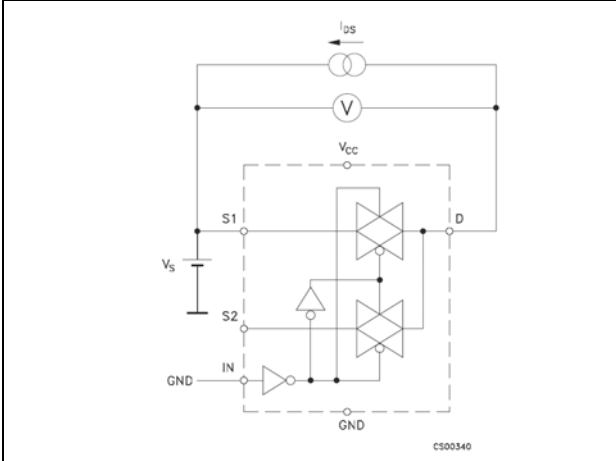
Figure 5. OFF leakage
