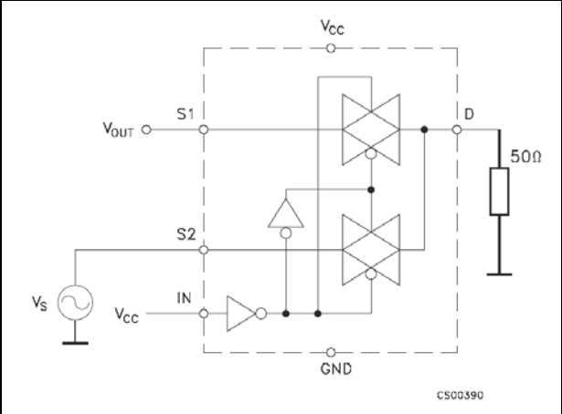
Figure 8. ON leakage
