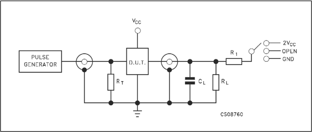
Figure 9. Test circuit
