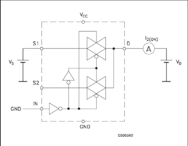
Figure 8. ON leakage
