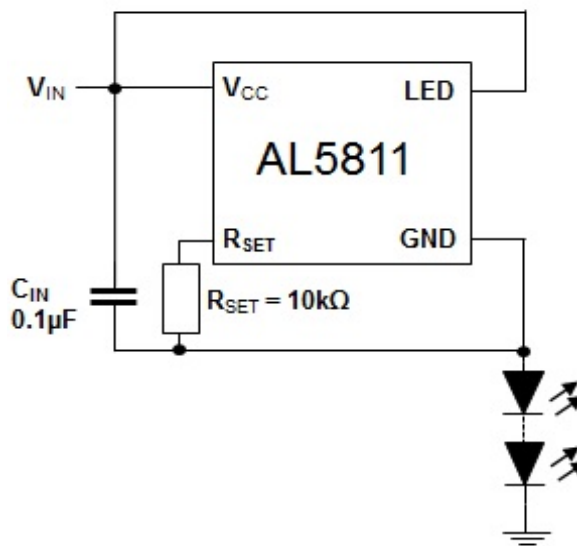
Figure 4. High Side Current LED String
