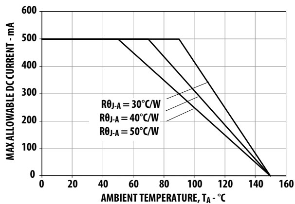
Figure 22. Maximum Forward Current vs. Ambient Temperature. Derated based on T_{JMAX} = 150\text{ }^{\circ}\text{C} , R_{\theta J-A} = 30\text{ }^{\circ}\text{C/W} , 40\text{ }^{\circ}\text{C/W} and 50\text{ }^{\circ}\text{C/W}
