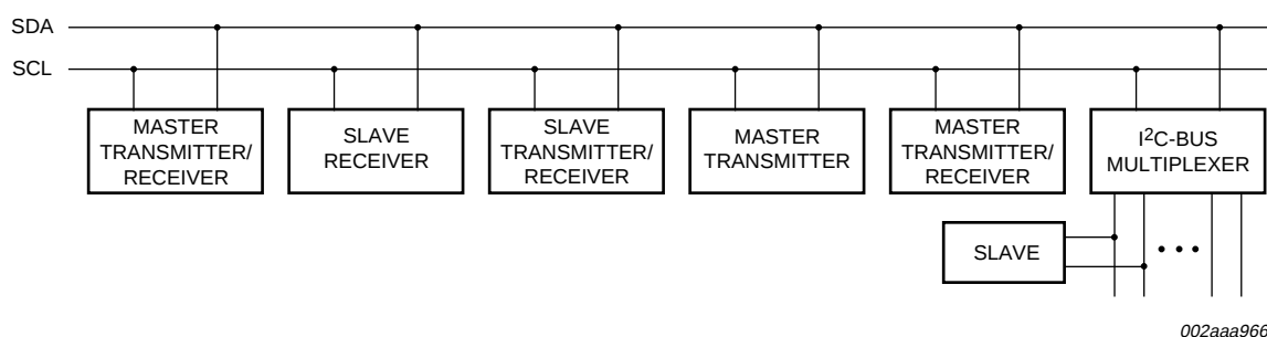
Fig 17. System configuration
