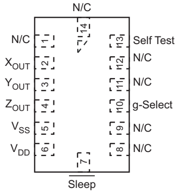
Figure 4. Pinout Description
