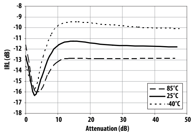
Figure 16. IRL vs Attenuation and Temperature at 450MHz
