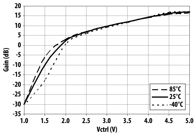
Figure 9. Gain vs Control Voltage and Temperature at 450MHz
