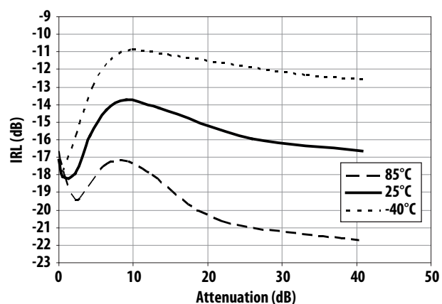
Figure 39. IRL vs Attenuation and Temperature at 900MHz
