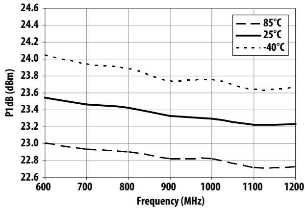
Figure 42. P1dB vs Frequency and Temperature at V_{ctrl} = 5\text{V}
