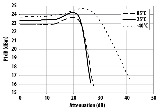
Figure 37. P1dB vs Attenuation and Temperature at 900MHz
