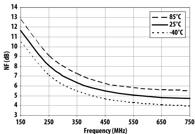
Figure 25. Noise Figure vs Frequency and Temperature at V_{ctrl} = 5\text{V}
