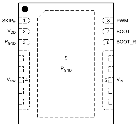
Figure 14. Top View
