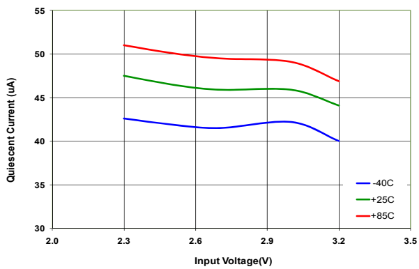
Figure 40. Quiescent Current
