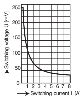
Safe disconnection, no remaining arc, max. 1 operation/sec. Maximum switching power curve
