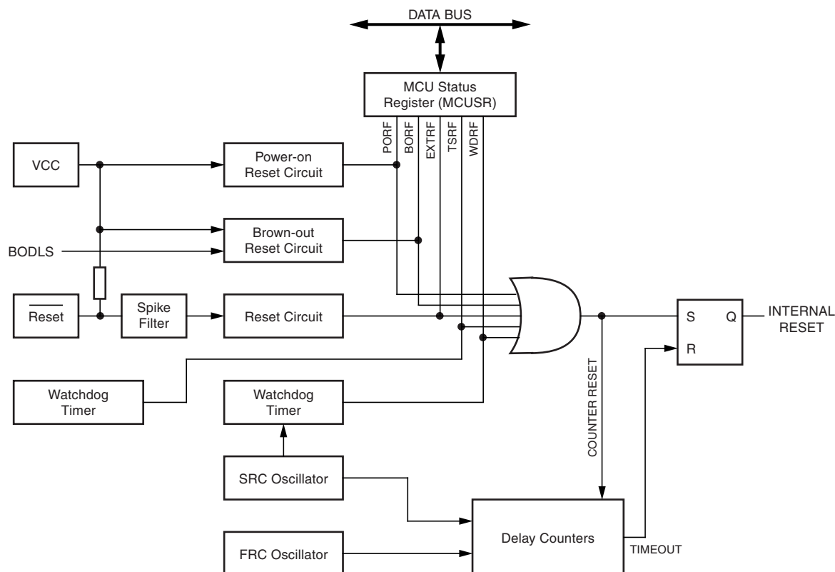
Figure 3-15. Reset Logic
