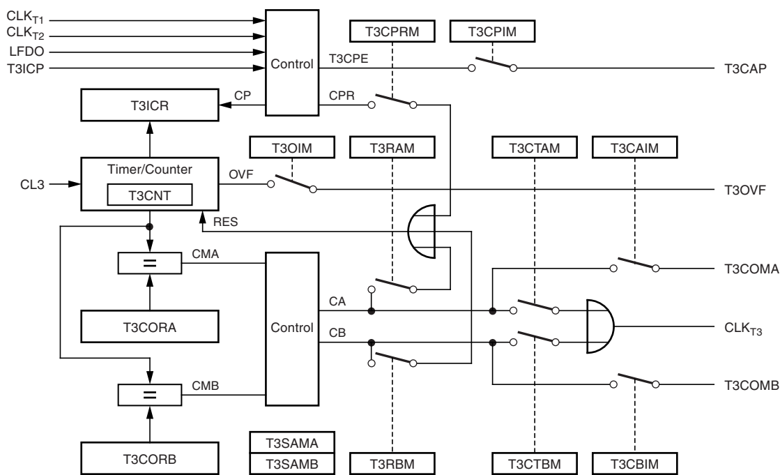
Figure 3-49. 16-Bit Counter3 Stage
