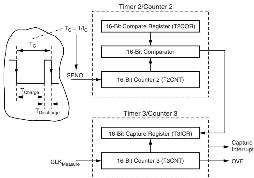
Timer 2/Counter 2
