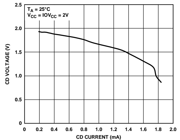
Figure 13. Carrier Detect—Voltage vs. Current, 2 V
