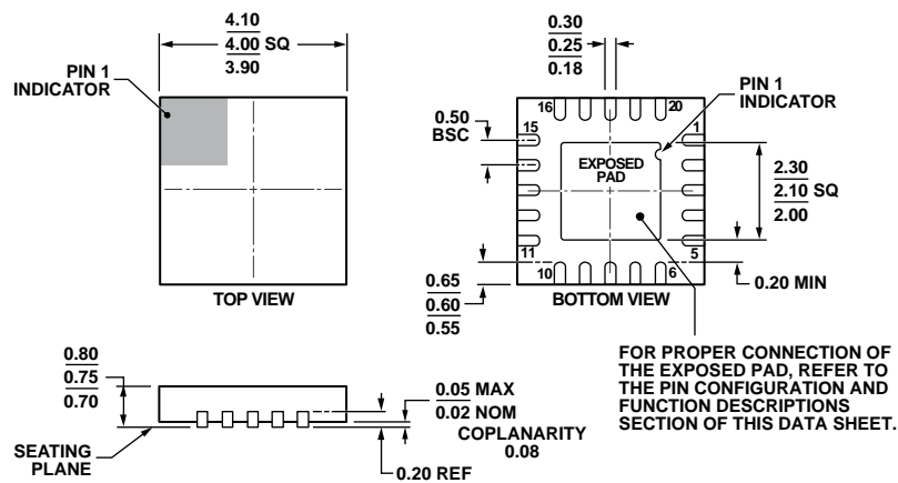
Figure 32. 20-Lead Lead Frame Chip Scale Package [LFCSP_WQ] 4 mm × 4 mm Body, Very Very Thin Quad
