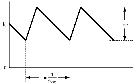
Figure 35. Inductor Current
