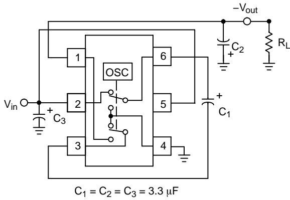
Figure 14. Test Setup/Voltage Inverter
