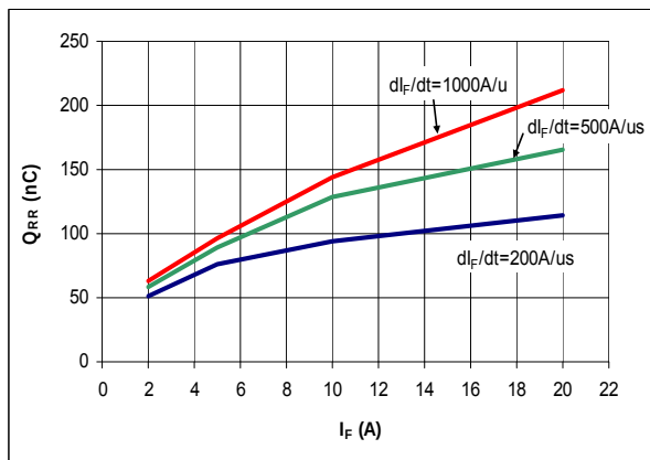
Figure 5. Typical Q_{rr} vs I_F at T_J = 125^\circ
