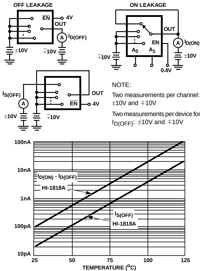
FIGURE 5. LEAKAGE CURRENTS vs TEMPERATURE
