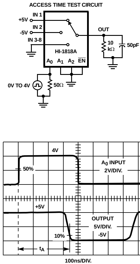
FIGURE 6. ACCESS TIME
