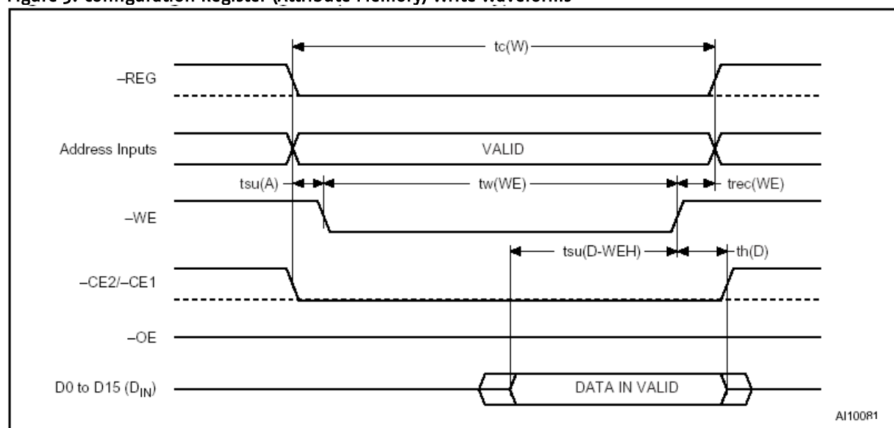
Figure 3: Configuration Register (Attribute Memory) Write waveforms
