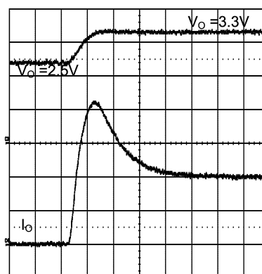
Figure 27. Pre-Biased Startup
