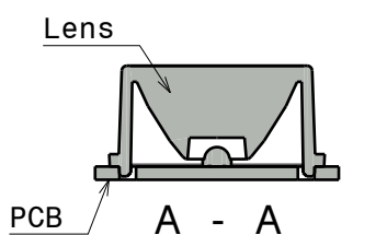
PCB suggestion
