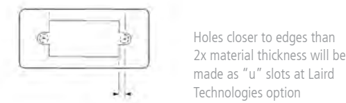
FIGURE 2B. SUB-D CONNECTOR
