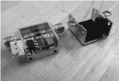
Figure 5. Amplifier and Enclosure with Lossy Foam Inside
