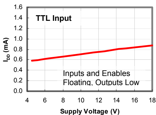
Figure 14. I_{DD} (Static) vs. Supply Voltage (15)
