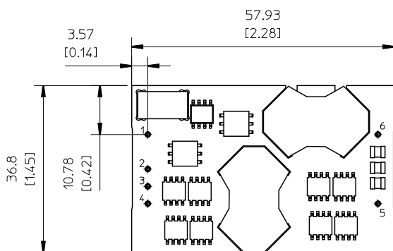
RECOMMENDED FOOTPRINT
