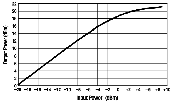
Figure 4. Output Power vs Input Power (f= 2.445 GHz, Vcc = 3.3 V, Tc = 25 °C)
