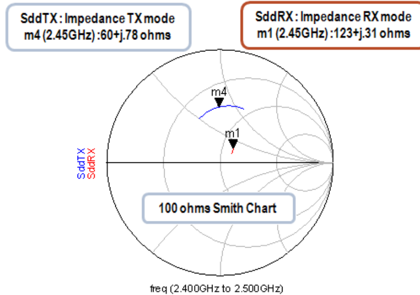
Figure 3. Transmit and Receive Differential Impedance (100 \Omega Reference)
