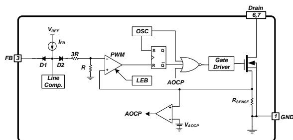
Figure 23. AOCP Circuit
