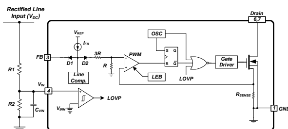
Figure 26. LOVP Circuit
