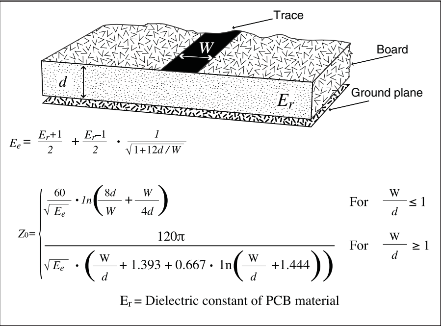
Figure 16: Microstrip Formulas
