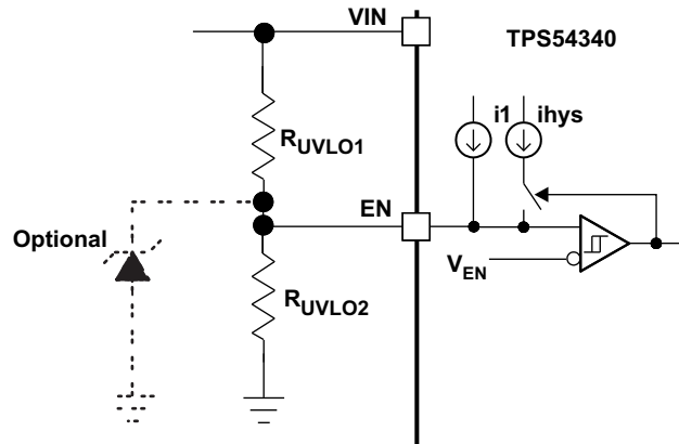
Figure 23. Adjustable Undervoltage Lockout (UVLO)
