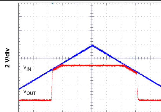
Time = 40 μs/div I_{OUT} = 1\text{ A} EN Floating
