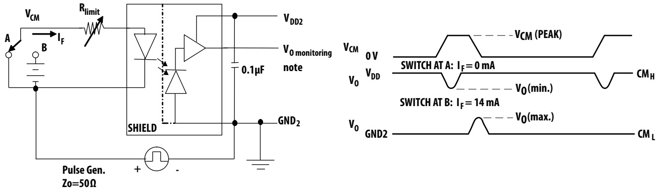
Figure 13. Test circuit for common mode transient immunity and typical waveforms. R_{\text{total}} is the total resistance of the driver output impedance (which is assumed to be 50 \Omega ) and the limiting resistor ( R_{\text{total}} = R_{\text{drv}} + R_{\text{limit}} ).
