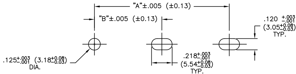
TYPICAL MOUNTING HOLES PANEL THICKNESS: .047-.085 (1.2-2.2)
