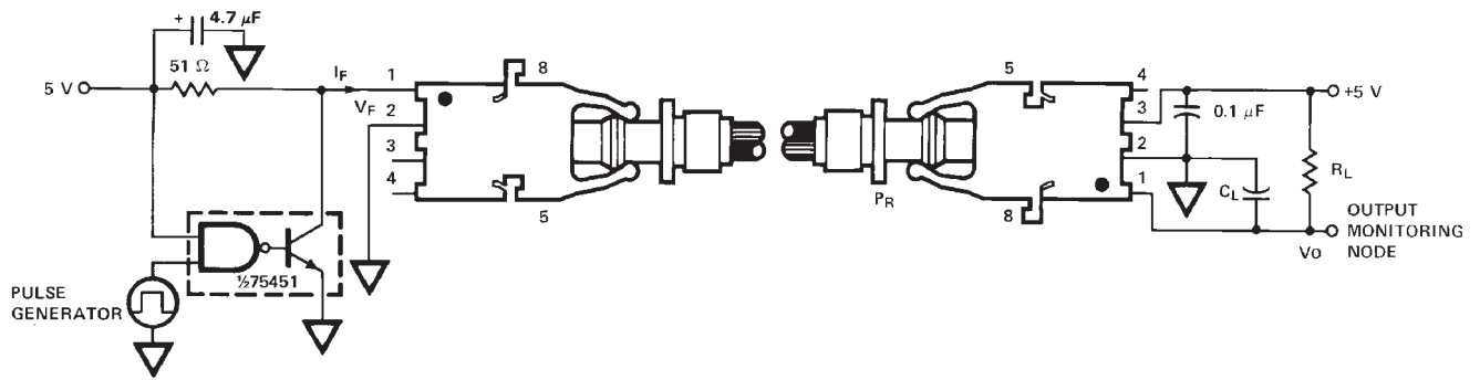
Figure 5. 5 Mb/s propagation delay test circuit
