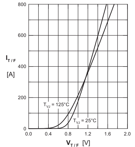
Fig. 1 Forward characteristics
