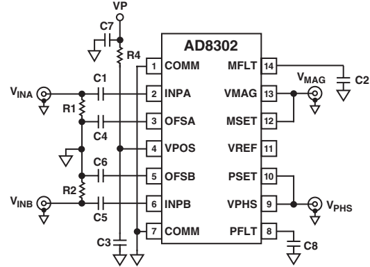
Figure 4. Basic Connections in Measurement Mode with 30\text{ mV/dB} and 10\text{ mV/Degree} Scaling
