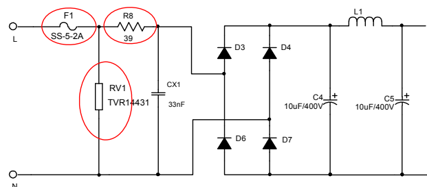
Figure 9: Solution to Pass 2kV Surge Test Layout Guide
