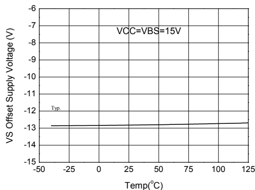
Figure 35. Maximum VS Negative Offset vs Temperature
