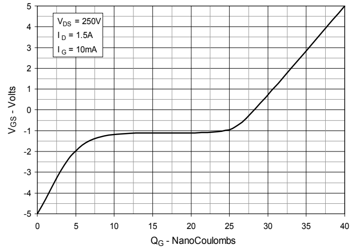
Fig. 14. Gate Charge
