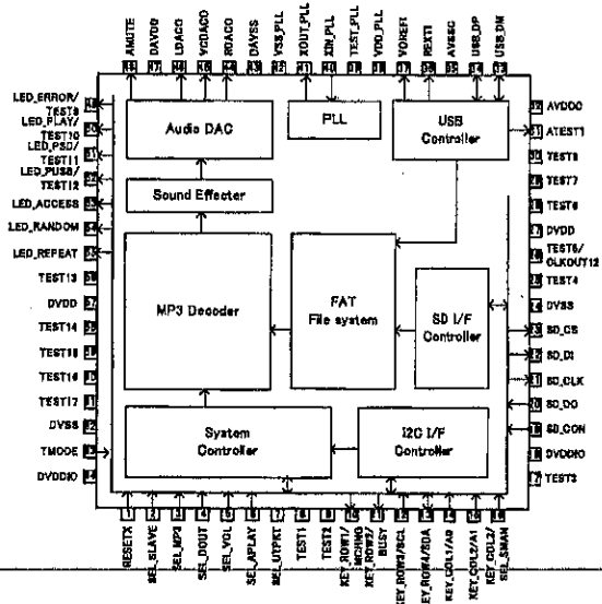
Figure 2. Block diagram
