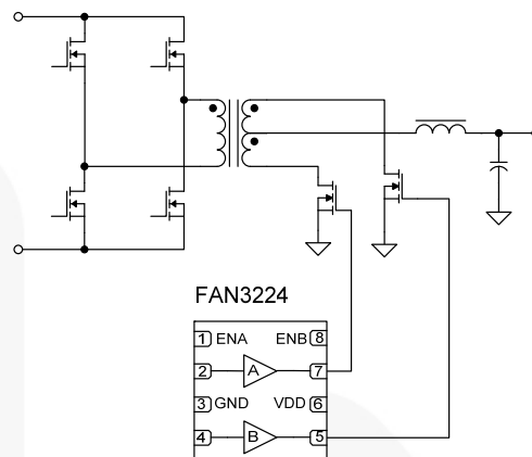
Figure 55. Center-Tapped Bridge Output with Synchronous Rectifiers
