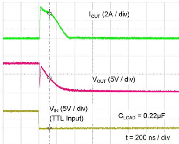
Figure 45. Quasi-Static Sink Current with V_{DD}=8\text{ V}^{(16)}
