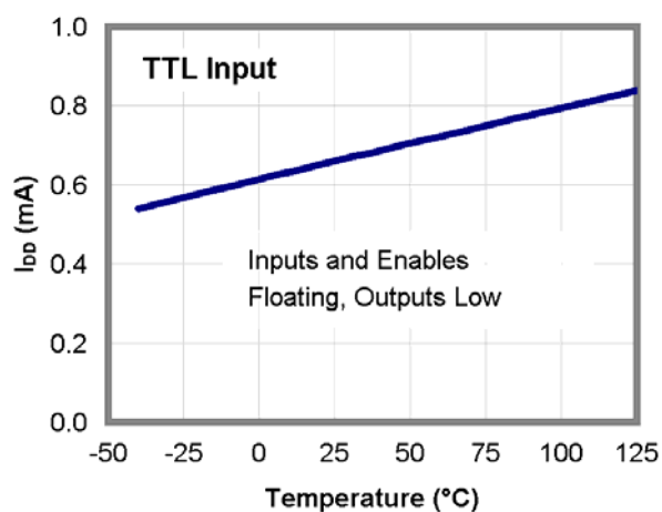
Figure 20. I_{DD} (Static) vs. Temperature (15)
