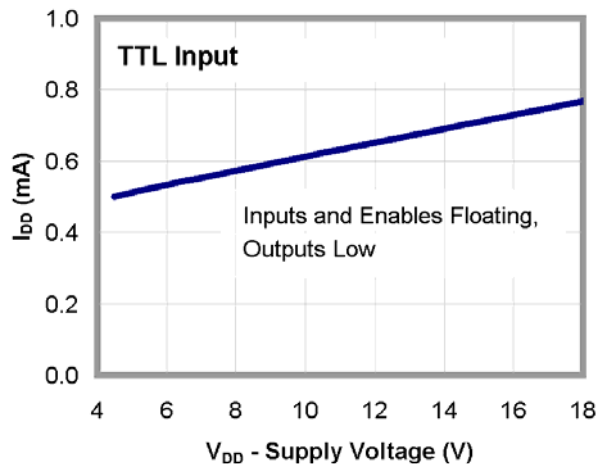
Figure 13. I_{DD} (Static) vs. Supply Voltage (15)
