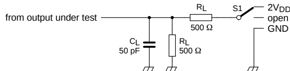
Figure 22. Load Circuit
