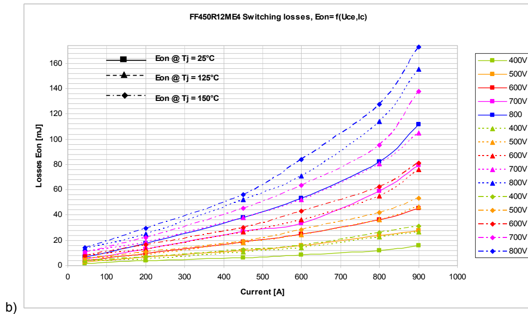
Figure 15 Turn-on losses with a) FF450R12ME3 and b) FF450R12ME4 module
