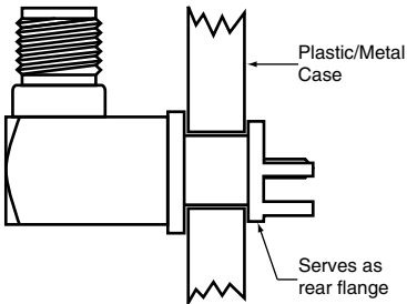
MOUNTING METHOD
