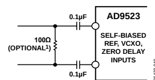
Figure 21. REF, VCXO, and Zero Delay Input Differential Mode
