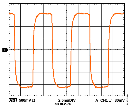
Figure 14. Output Waveform (Differential), HSTL at 16 mA, 122.88 MHz
