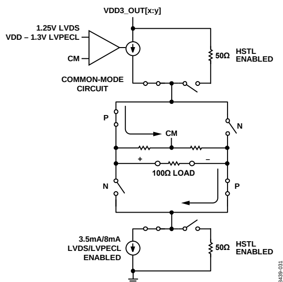
Figure 26. Multimode Driver
