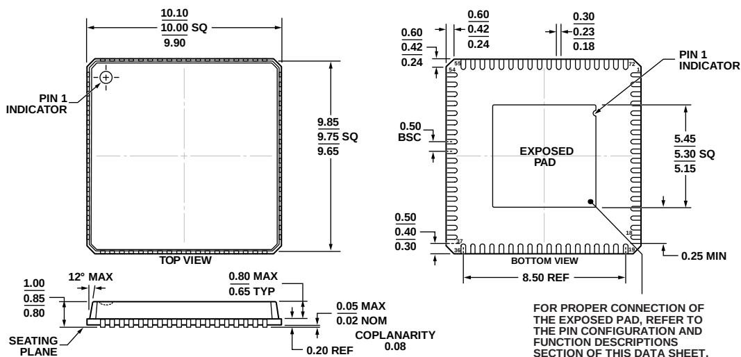
Figure 45. 72-Lead Lead Frame Chip Scale Package [LFCSP_VQ] 10 mm × 10 mm Body, Very Thin Quad (CP-72-6)
