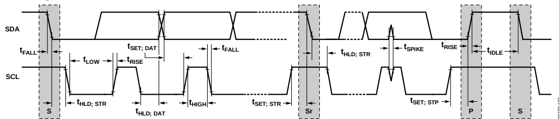
Figure 35. I 2 C Serial Port Timing
