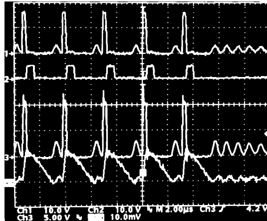
Figure 11. Normal SKIP Mode Operation at Light Loads
