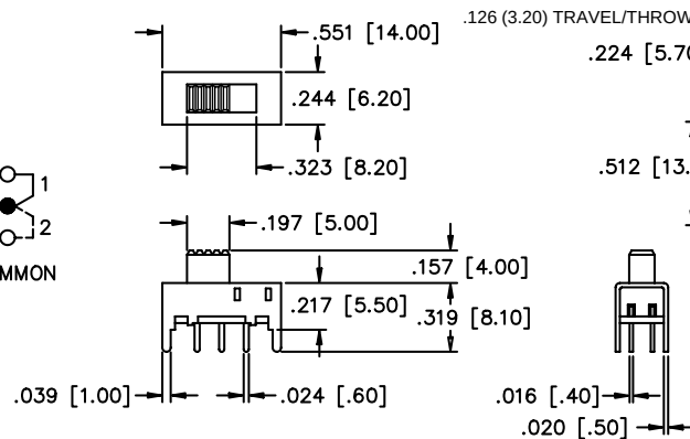
MECHANICAL OUTLINE
