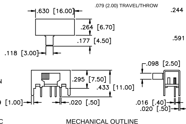
MECHANICAL OUTLINE
