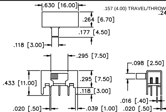
MECHANICAL OUTLINE
