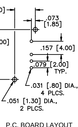
P.C. BOARD LAYOUT
