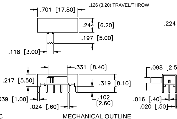
MECHANICAL OUTLINE
