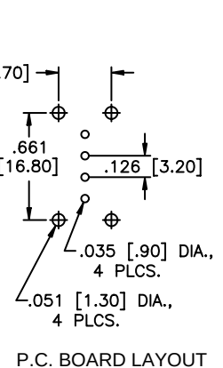
P.C. BOARD LAYOUT
